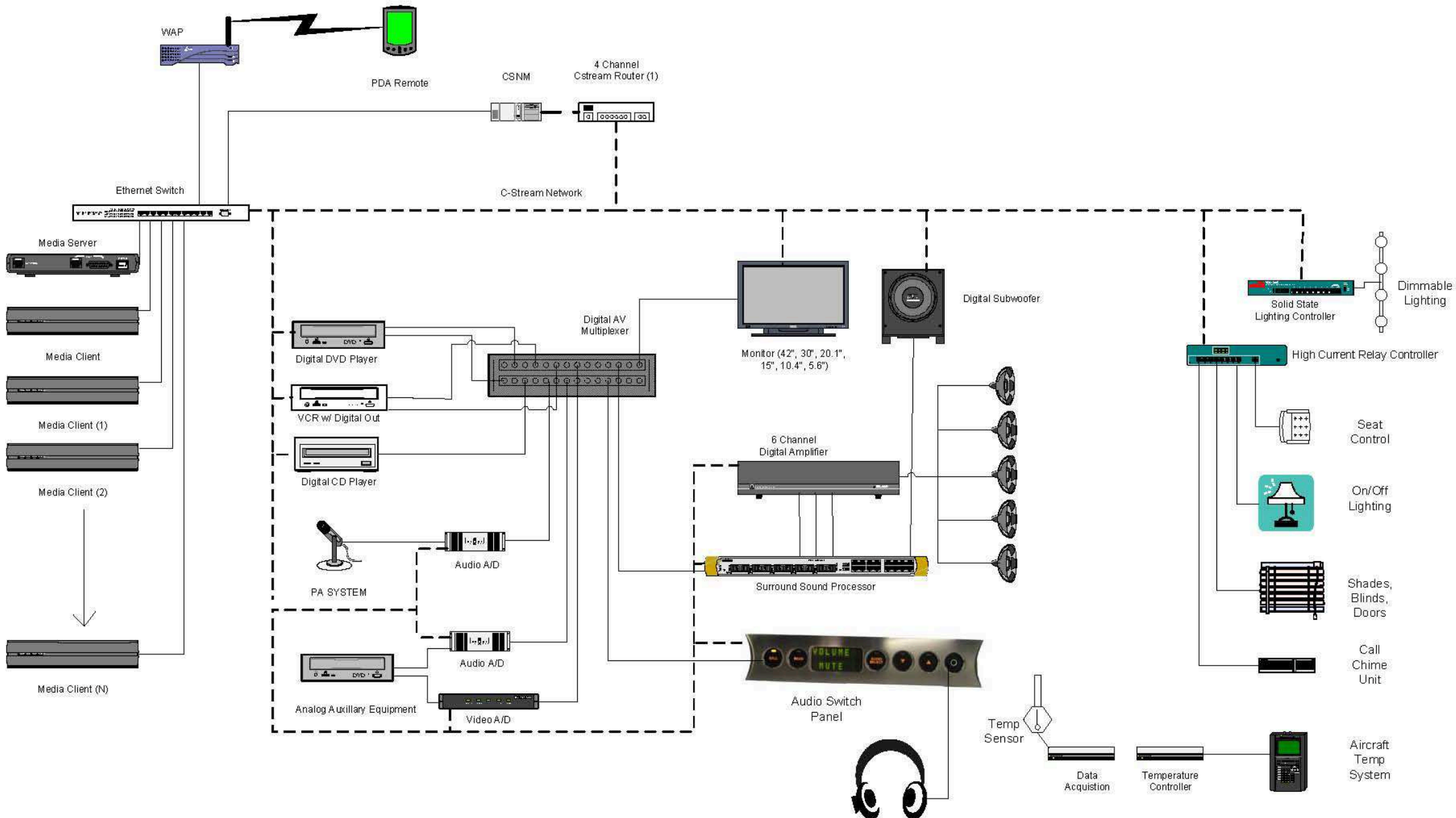
AVOD SYSTEM
